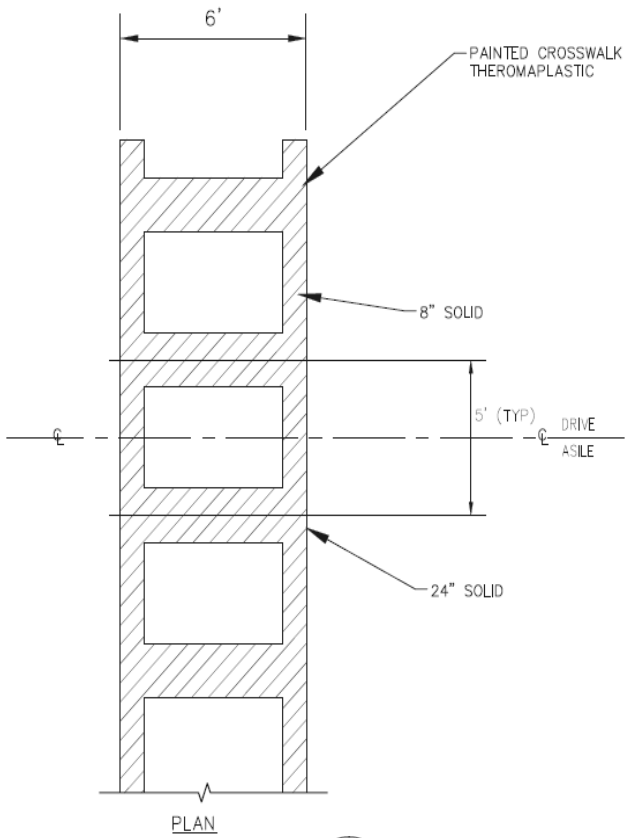
STRIPED WALKWAY SW NTS
