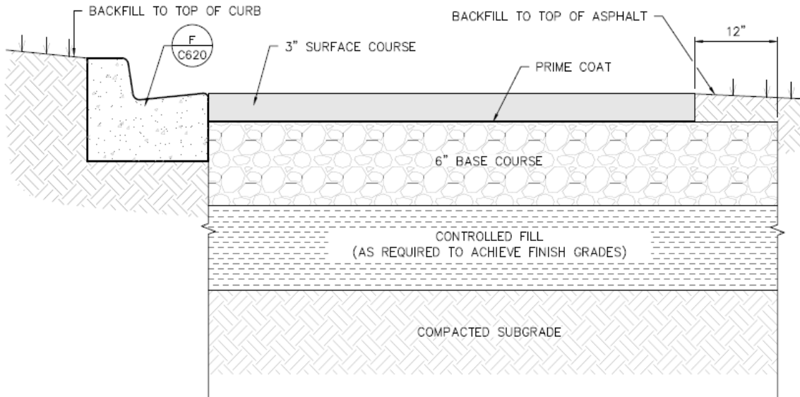
A STANDARD DUTY ASPHALTIC CONCRETE PAVEMENT SECTION
