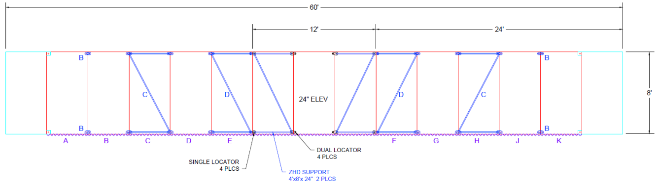
A PLAN VIEW - RAMP 0-24" SCALE: NONE
